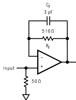
FIGURE 1. Typical Circuit for A_V = +1 Operation ( V_S \geq 6\text{V} )
